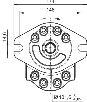
Type flange SAEB-T13
