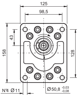
Type flange 3-C9
